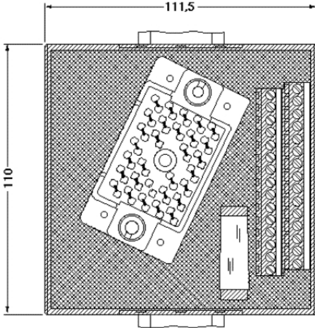
Dimensioned drawing
