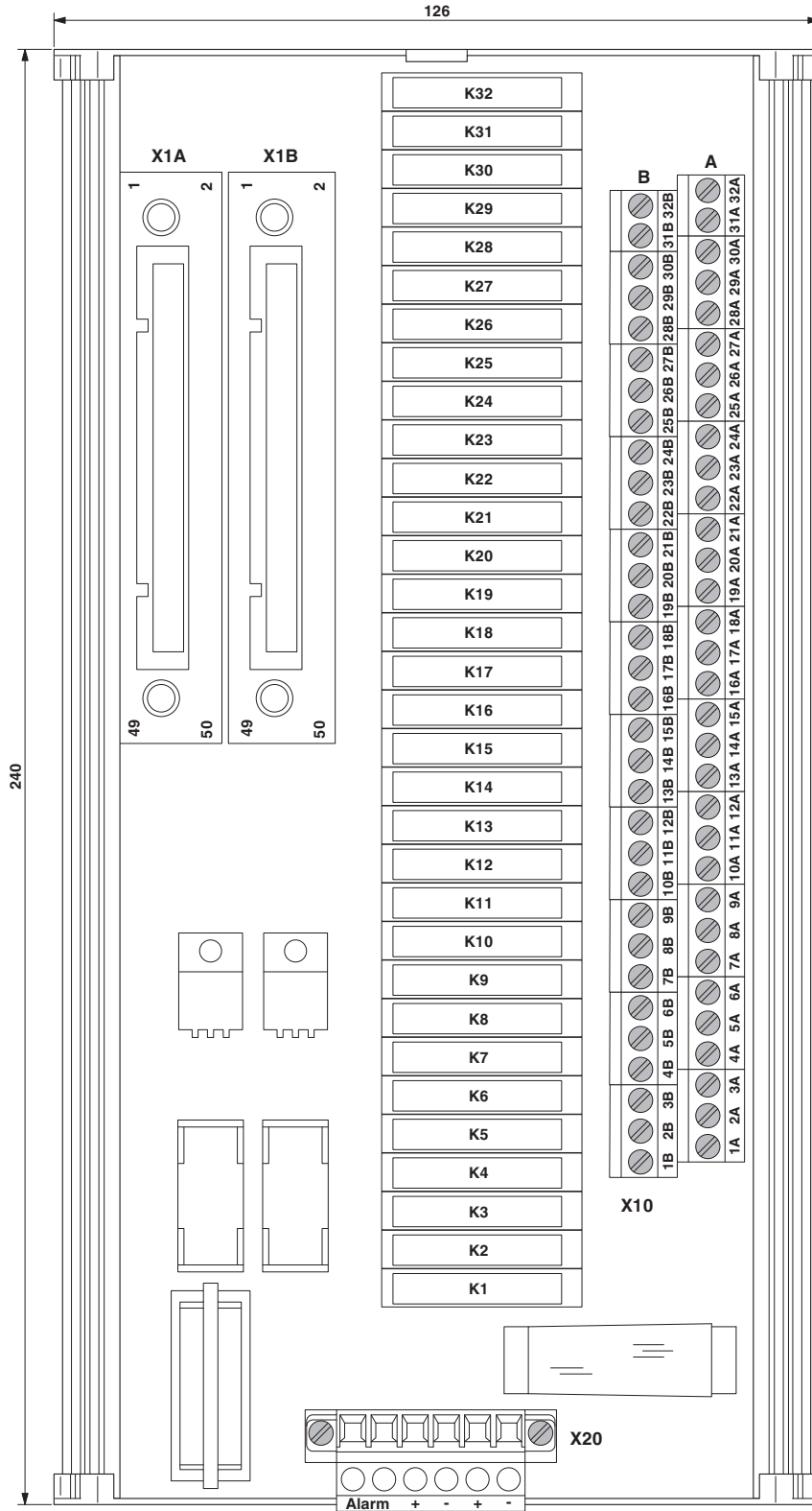
Dimensional drawing
