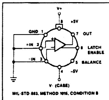
STANDARD BURN-IN CIRCUIT
