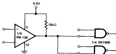
DRIVING TTL
