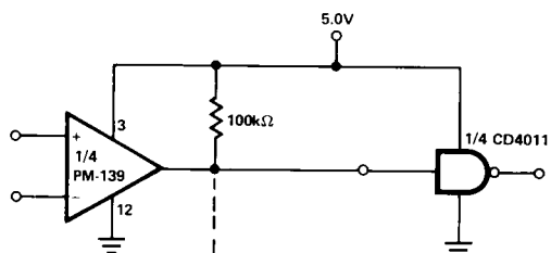
DRIVING CMOS
