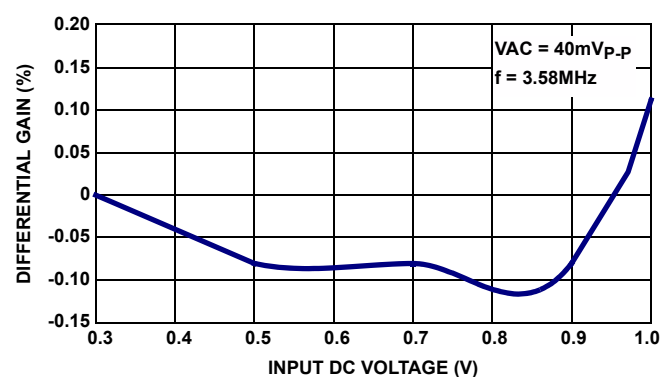
FIGURE 17. DIFFERENTIAL GAIN
