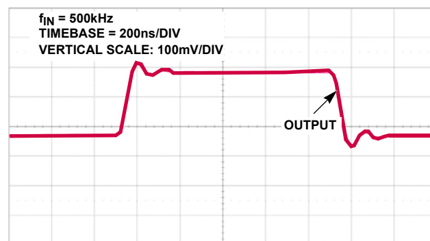
FIGURE 12. SMALL SIGNAL PULSE RESPONSE
