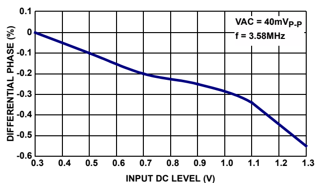
FIGURE 18. DIFFERENTIAL PHASE
