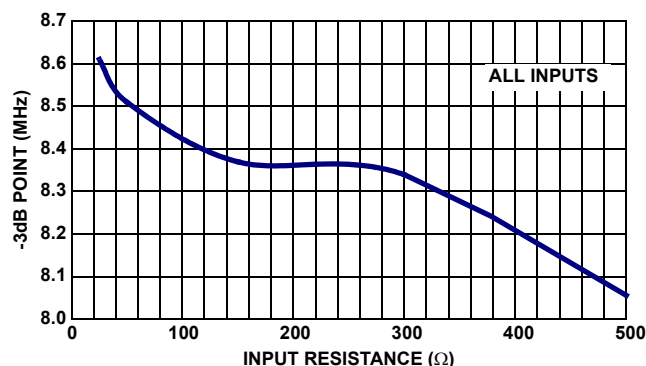
FIGURE 22. -3dB BANDWIDTH vs INPUT RESISTANCE
