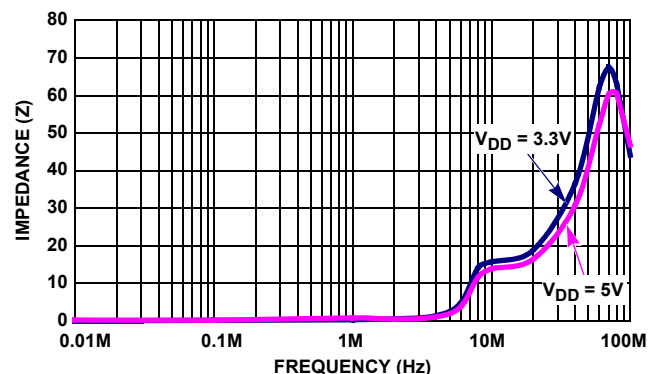
FIGURE 7. OUTPUT IMPEDANCE vs FREQUENCY
