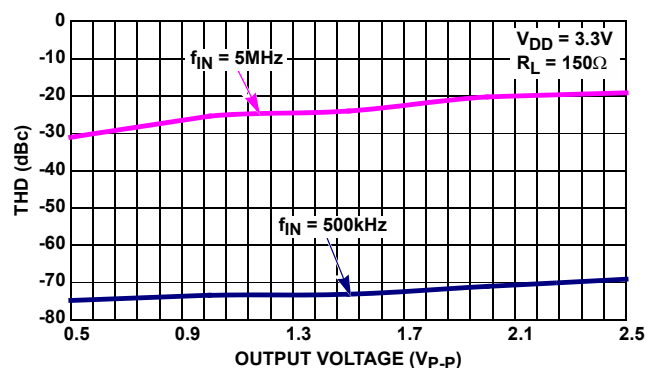
FIGURE 20. TOTAL HARMONIC DISTORTION vs OUTPUT VOLTAGE
