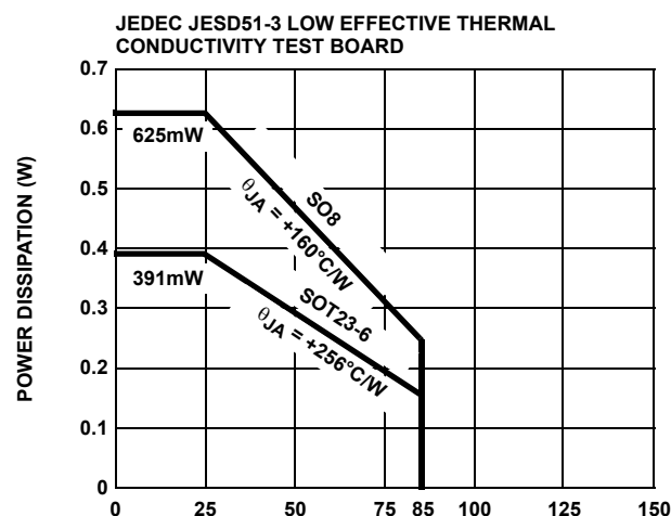
FIGURE 26. PACKAGE POWER DISSIPATION vs AMBIENT TEMPERATURE
