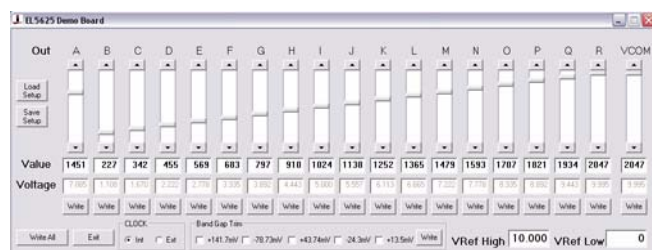
FIGURE 7. USB INTERFACE
