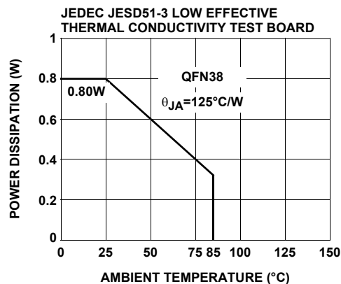
FIGURE 6. PACKAGE POWER DISSIPATION vs AMBIENT TEMPERATURE
