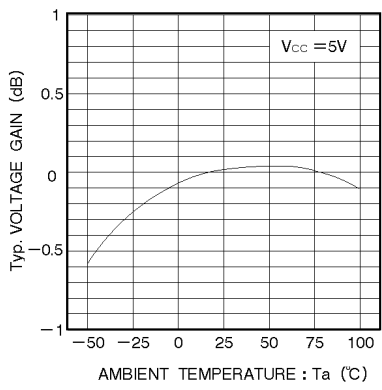
Fig.7 Voltage gain vs temperature
