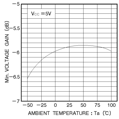
Fig.8 Minimum voltage gain vs temperature
