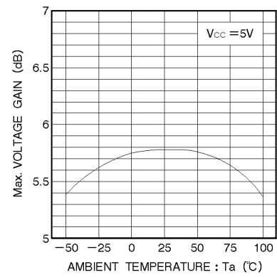
Fig.6 Maximum voltage gain vs temperature
