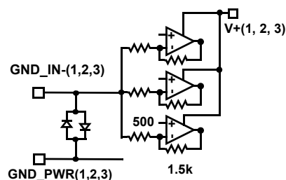
CIRCUIT 4
