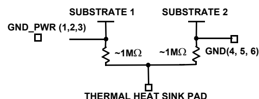
CIRCUIT 6
