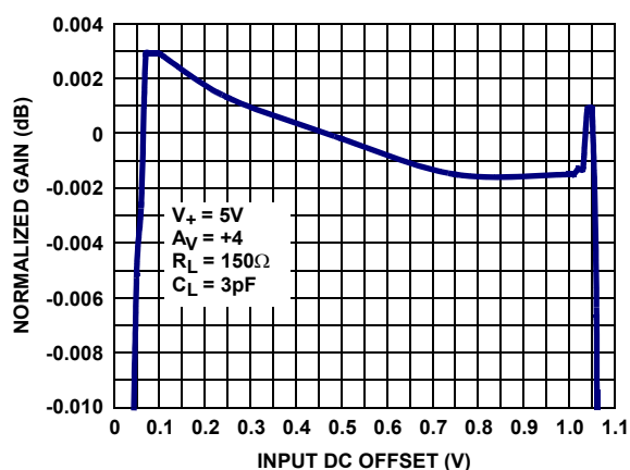
FIGURE 16. DIFFERENTIAL GAIN
