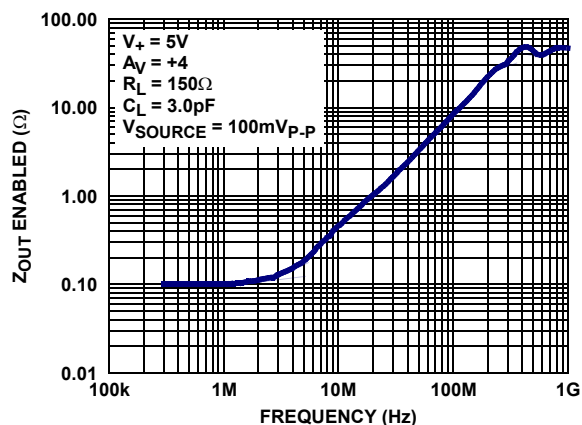
FIGURE 19. Z_{OUT} (ENABLED) vs FREQUENCY
