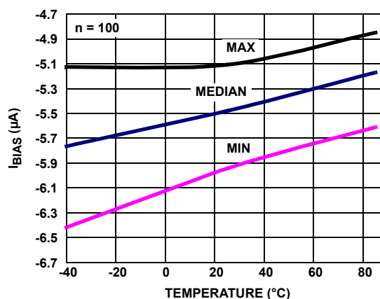
FIGURE 24. I_{BIAS} vs TEMPERATURE, V_S = \pm 2.5V
