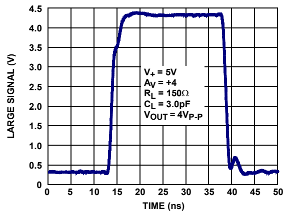
FIGURE 15. LARGE SIGNAL (4V P-P ) STEP RESPONSE
