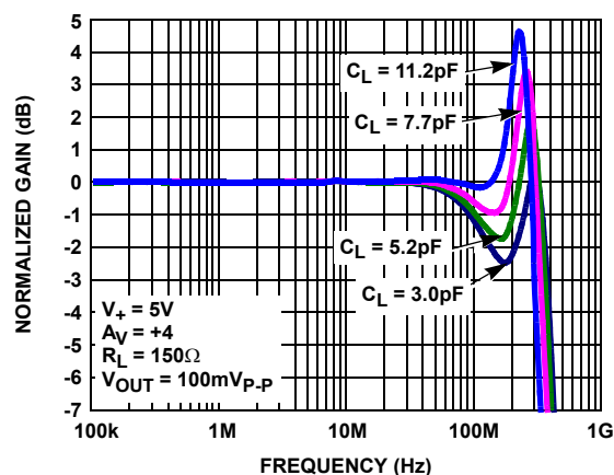
FIGURE 3. GAIN vs FREQUENCY FOR VARIOUS C_{LOAD}
