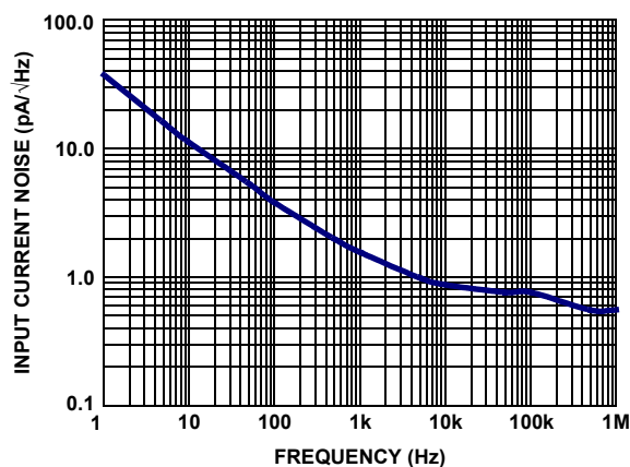
FIGURE 11. INPUT REFERRED NOISE CURRENT vs FREQUENCY
