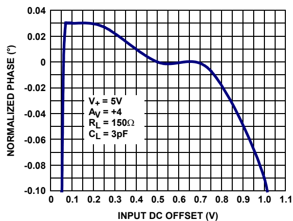
FIGURE 17. DIFFERENTIAL PHASE
