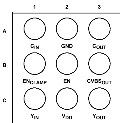
ISL59116 (WLCSP) TOP VIEW
