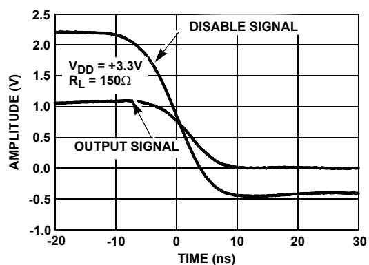
FIGURE 14. DISABLE TIME
