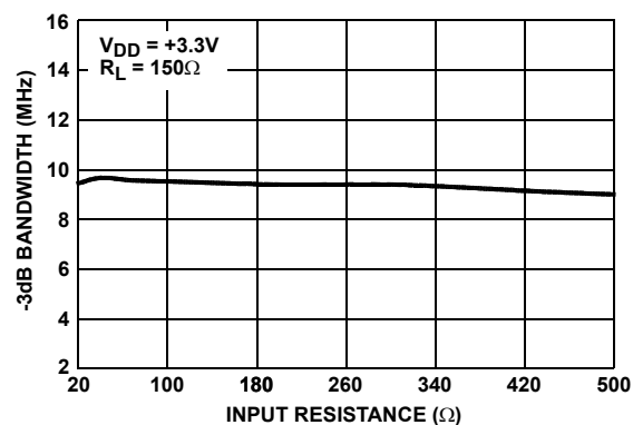
FIGURE 18. -3dB BANDWIDTH vs INPUT RESISTANCE
