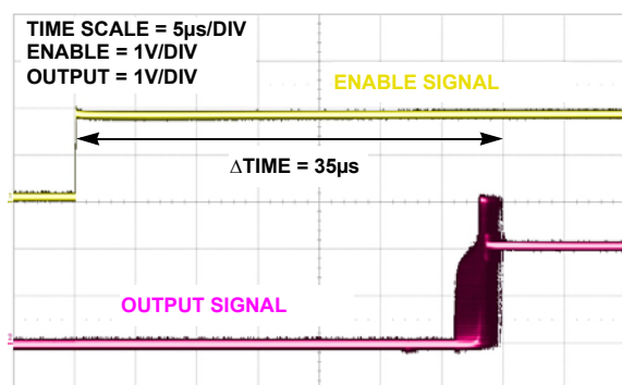
FIGURE 15. ENABLE TIME
