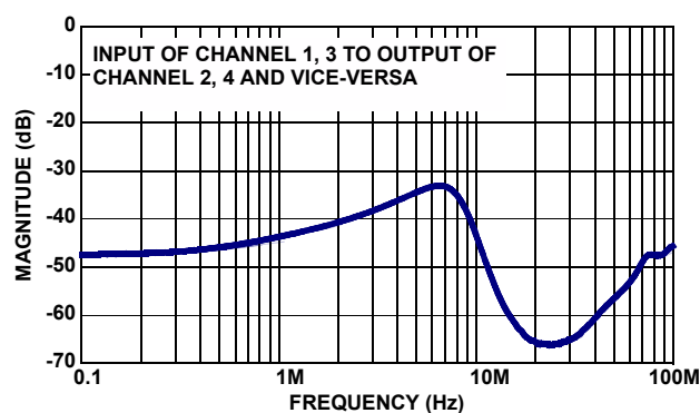
FIGURE 7. LUMA-TO-CHROMA CROSSTALK
