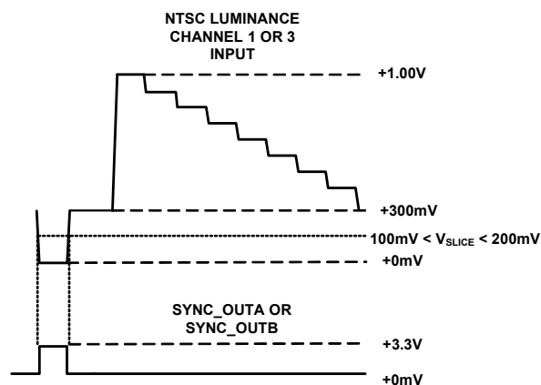
FIGURE 29. SYNC DETECTOR SLICE LEVEL
