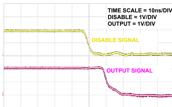
FIGURE 14. DISABLE TIME
