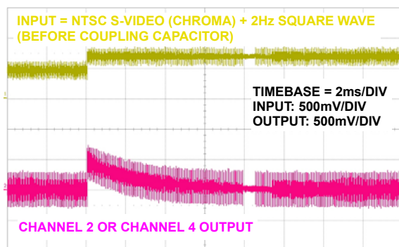
FIGURE 23. CHROMA CLAMP RESPONSE TO POSITIVE TRANSIENT (CHANNEL 2 AND 4)
