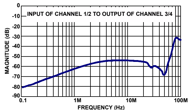
FIGURE 6. INTER-CHANNEL CROSSTALK
