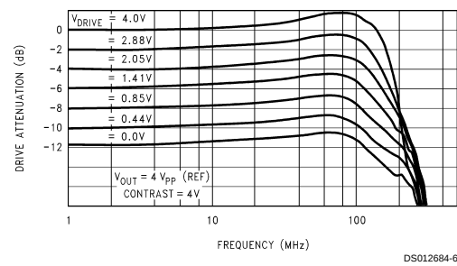
LM1283 Drive vs Frequency
