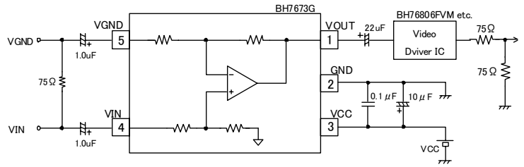
Fig.2 Application circuit examples
