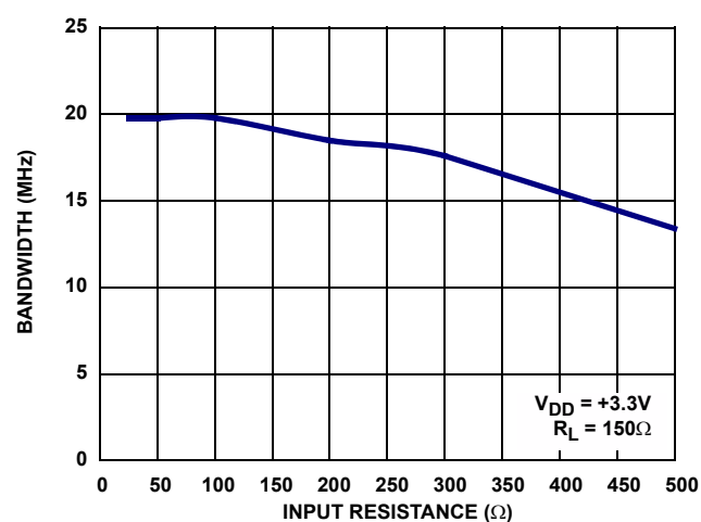
FIGURE 18. -3dB BANDWIDTH vs INPUT RESISTANCE
