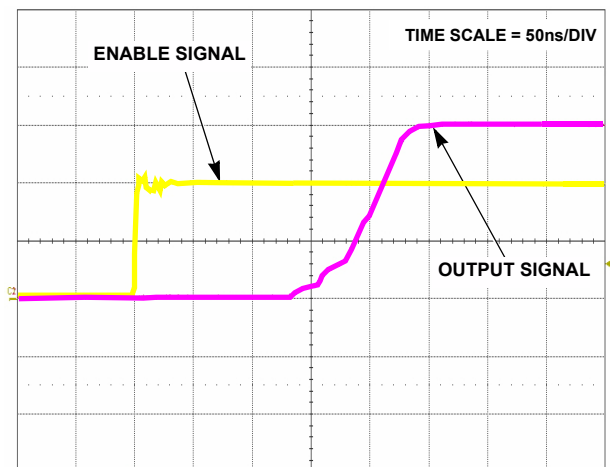
FIGURE 13. ENABLE TIME
