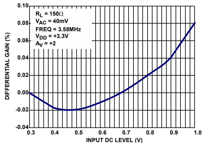
FIGURE 20. DIFFERENTIAL GAIN
