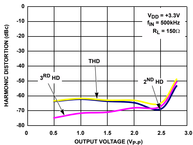
FIGURE 16. HARMONIC DISTORTION vs OUTPUT VOLTAGE
