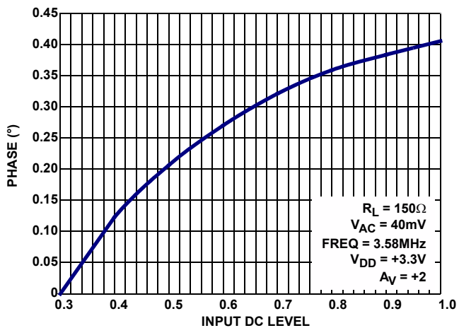
FIGURE 21. DIFFERENTIAL PHASE
