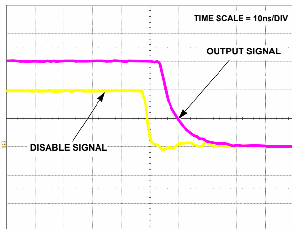
FIGURE 14. DISABLE TIME
