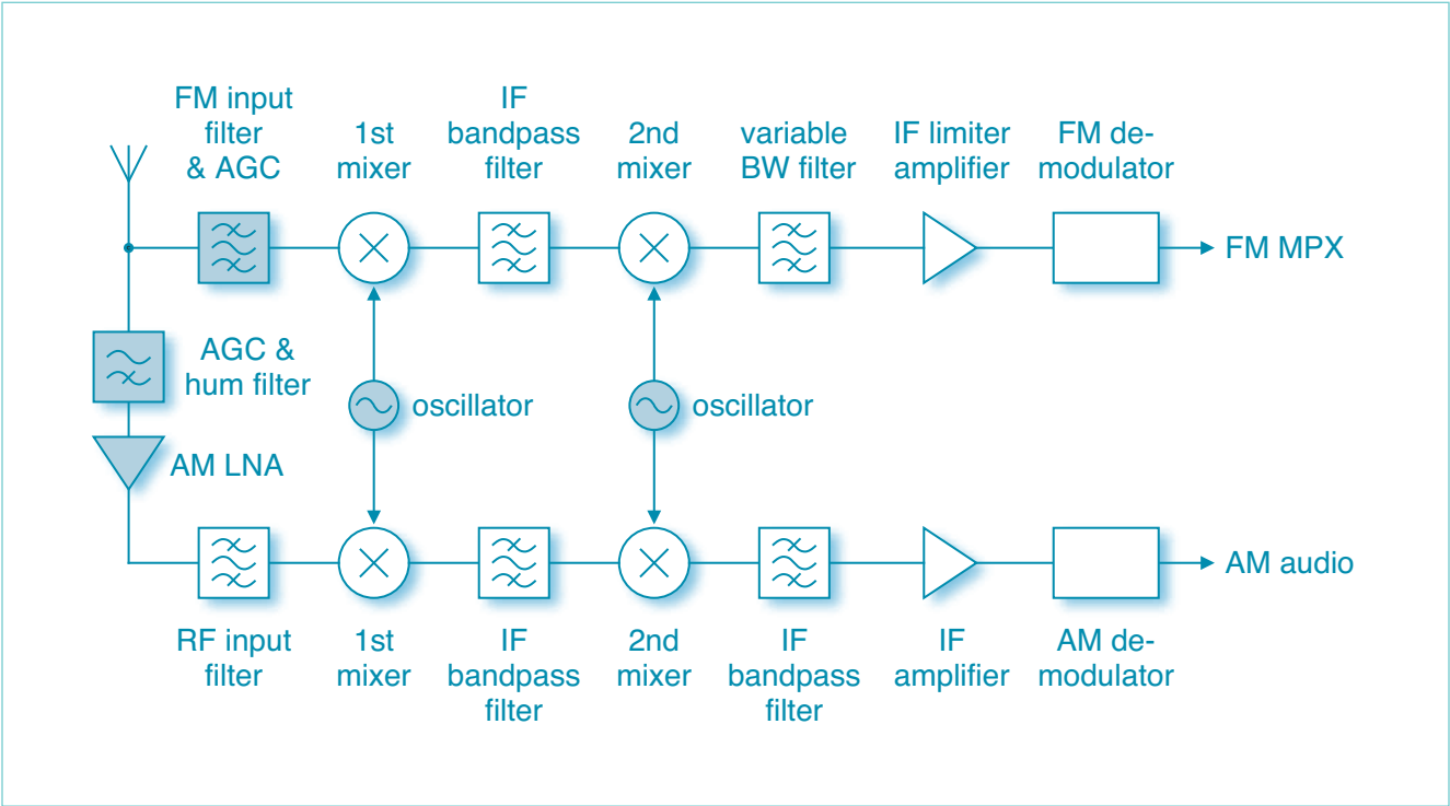
Application diagram
