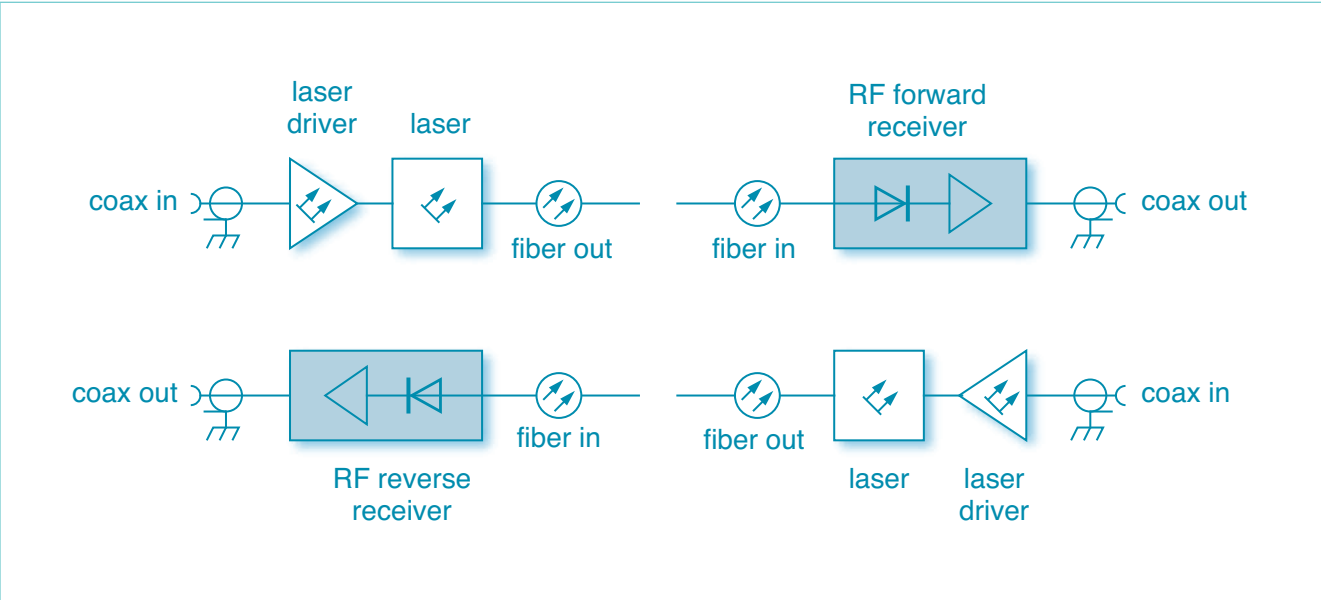
Application diagram
