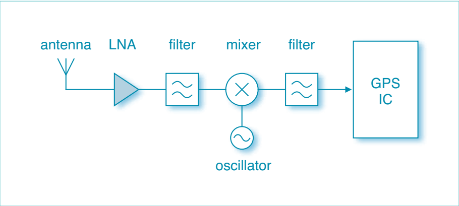
Application diagram
