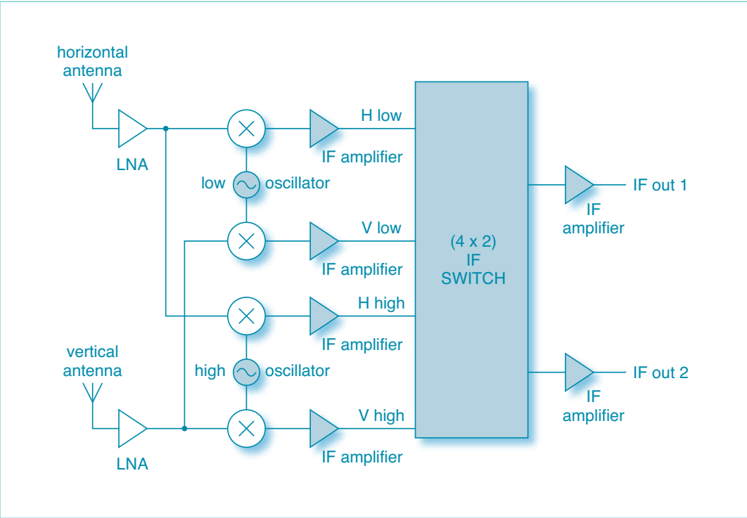
Application diagram
