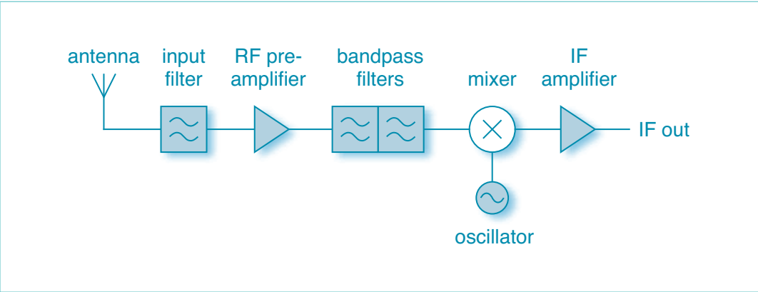
Application diagram
