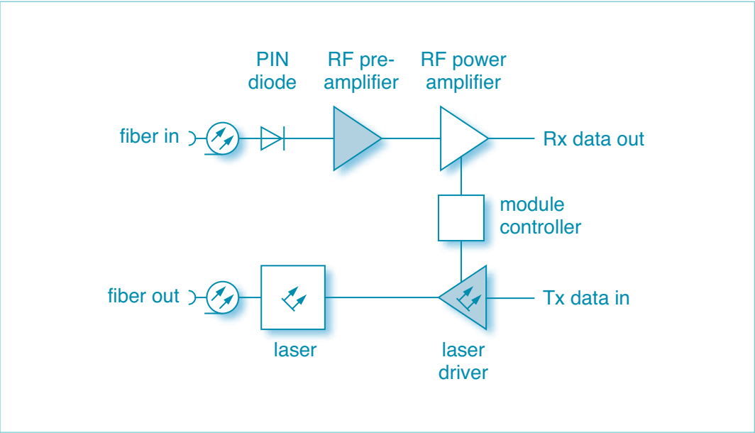
Application diagram
