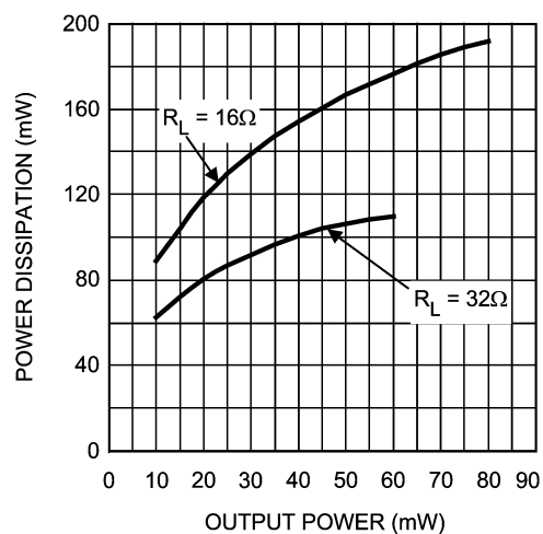
Power Dissipation vs Output Power V_{DD} = 3V
