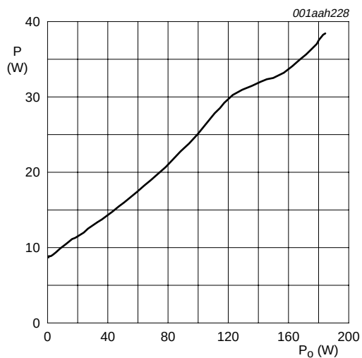
Fig 32. Power dissipation as a function of output power (one channel), SE application
