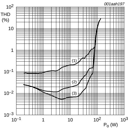
V_P = \pm 27 V; double coils; C = 680 nF. (1) f = 10 kHz. (2) f = 1 kHz. (3) f = 100 Hz. a. R_L = 4 \Omega .
