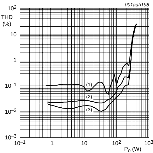
V_P = \pm 27 V; double coils; C = 680 nF. (1) f = 10 kHz. (2) f = 1 kHz. (3) f = 100 Hz. b. R_L = 4 \Omega
