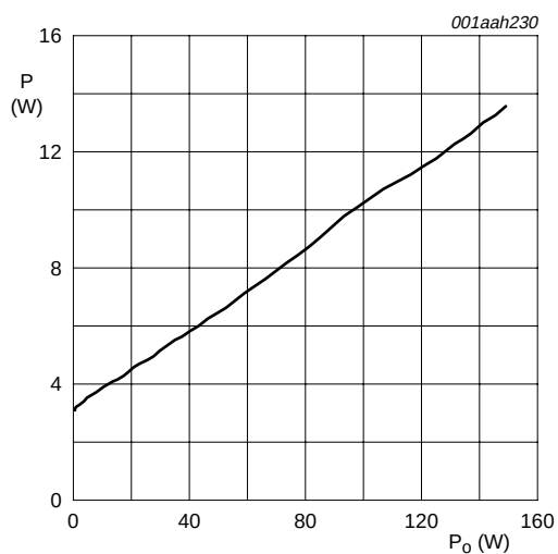
Fig 33. Power dissipation as a function of output power, BTL application
