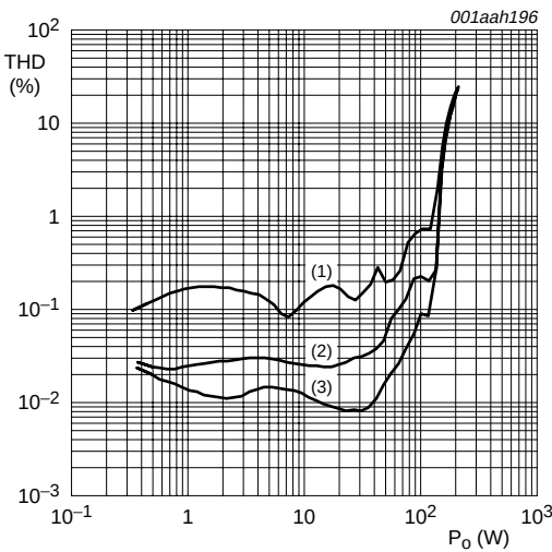
V_P = \pm 27 V; double coils; C = 680 nF. (1) f = 10 kHz. (2) f = 1 kHz. (3) f = 100 Hz. b. R_L = 2 \Omega .
