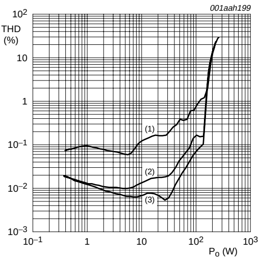
V_P = \pm 27 V; double coils; C = 680 nF. (1) f = 10 kHz. (2) f = 1 kHz. (3) f = 100 Hz. a. R_L = 8 \Omega
