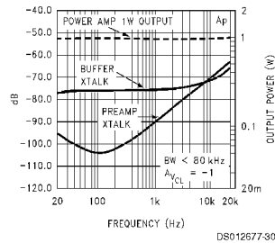
Power Amp Crosstalk to Preamp and Buffer
