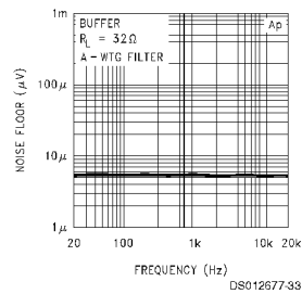
Wideband Noise Floor
