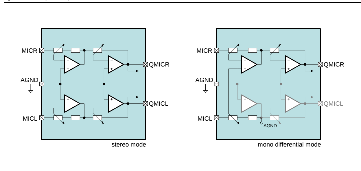
Figure 18. Microphone Input
