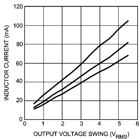
Inductor Current vs Output Voltage Swing
