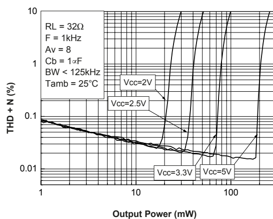
Figure 82. THD + N vs. output power R_L = 32\ \Omega , A_v = 8
