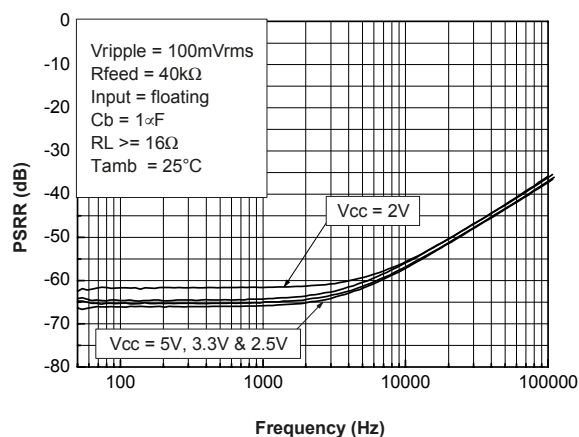
Figure 72. PSRR vs. power supply voltage
