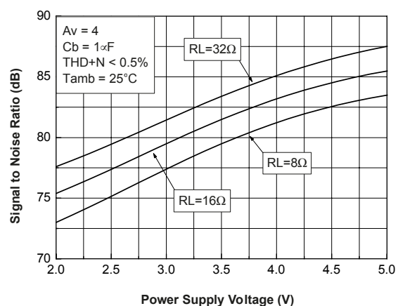
Figure 68. Signal-to-noise ratio vs. power supply voltage with unweighted filter (20 Hz to 20 kHz)
