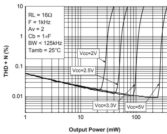
Figure 39. THD + N vs. output power R_L = 16 \Omega , A_v = 2
