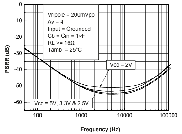
Figure 74. PSRR vs. bypass capacitor C_b = C_{in} = 1\mu\text{F}
