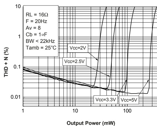
Figure 78. THD + N vs. output power R_L = 16\ \Omega
