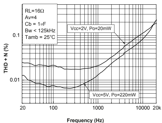
Figure 66. THD + N vs. frequency R_L = 16\ \Omega
