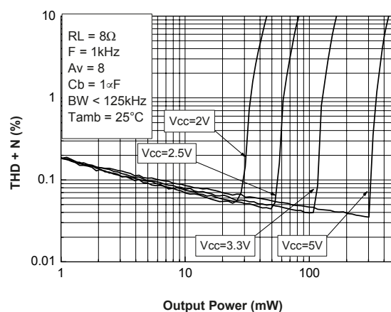
Figure 80. THD + N vs. output power R_L = 8\ \Omega , A_v = 8
