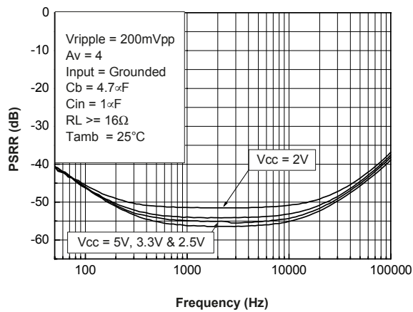
Figure 75. PSRR vs. bypass capacitor C_b = C_{in} = 4.7\mu\text{F}
