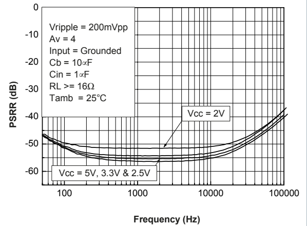
Figure 76. PSRR vs. bypass capacitor C_b = C_{in} = 10\mu\text{F}
