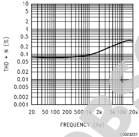
THD+N vs Frequency at V_{DD} = 3V , 4\Omega R_L , and PWR = 225mW
