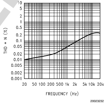
THD+N vs Frequency V_{DD} = 2.6V , 8\Omega R_L , and PWR = 150mW
