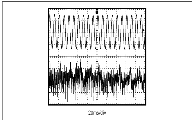
Figure 5. RMS Comparison of Sine Wave vs. Audio Signal
