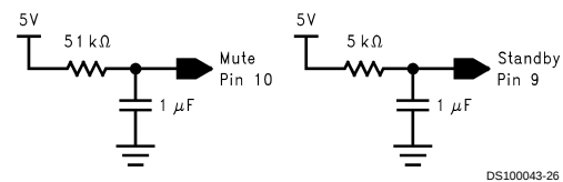
FIGURE 2. Mute and Standby Pin Lowpass Filters
