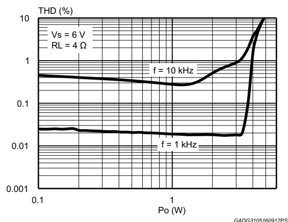
Figure 10. Distortion vs. output power (4 \Omega , V_s = 6 \text{ V} )
