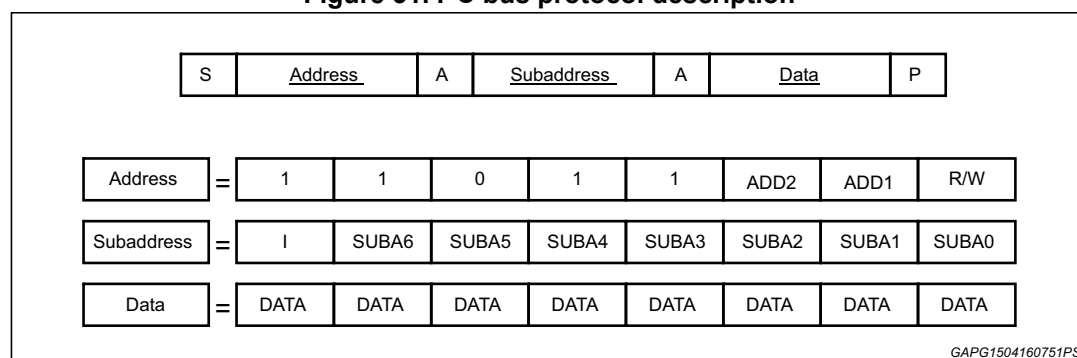
Figure 31. I 2 C bus protocol description
