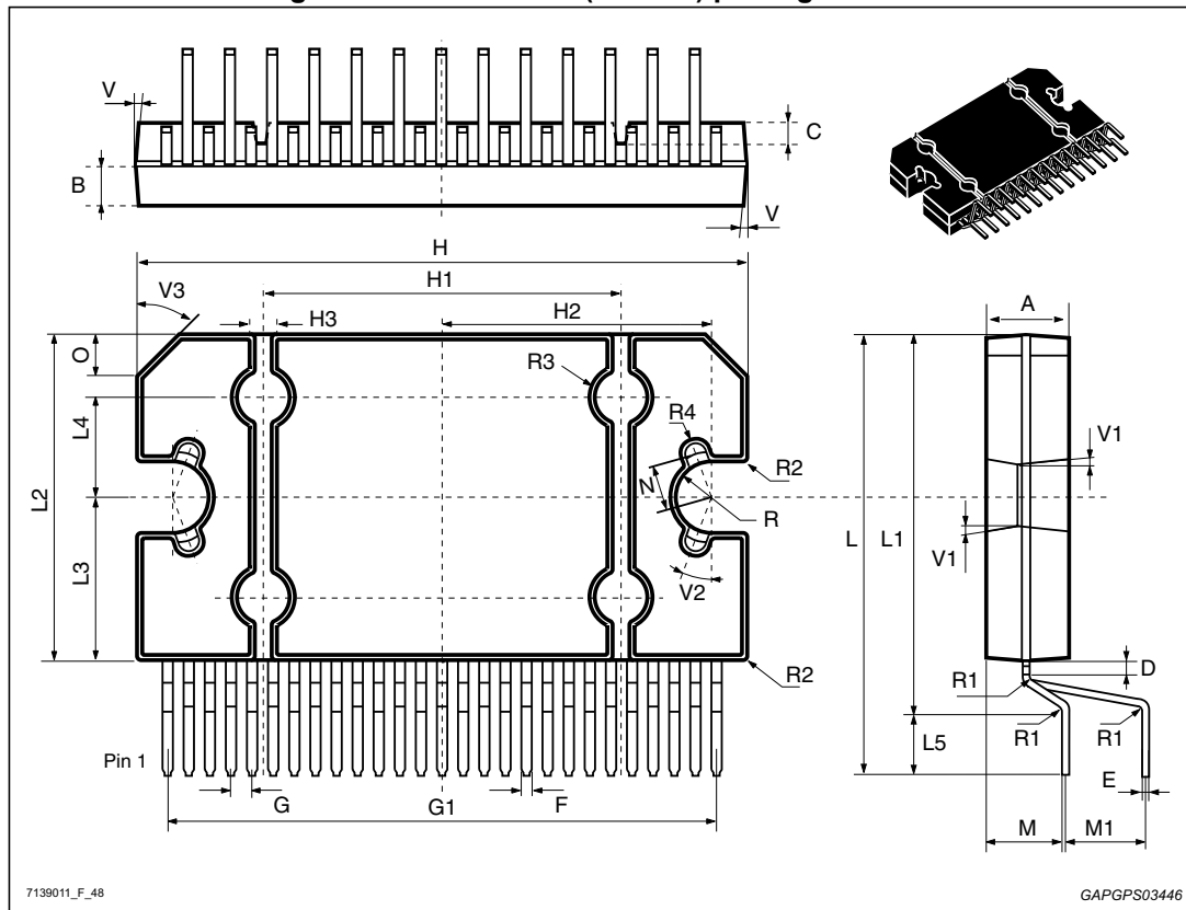
Figure 34. Flexiwatt 27 (vertical) package outline
