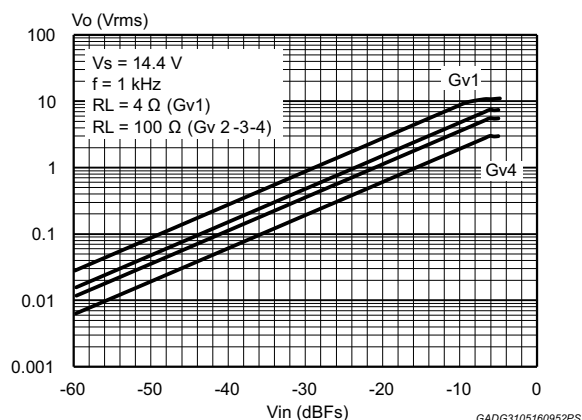
Figure 11. V_o vs. V_{in} (Gv1-2-3-4 settings)
