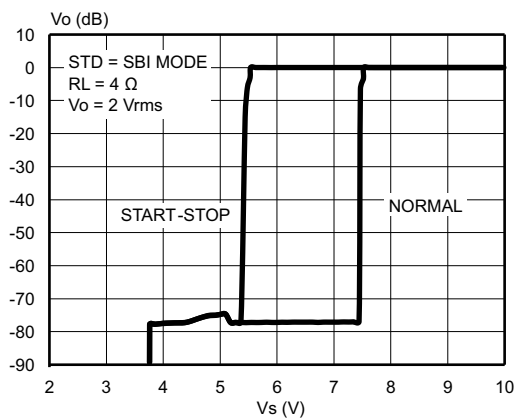
Figure 16. Output attenuation vs. supply voltage
