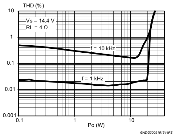
Figure 7. Distortion vs. output power (4 \Omega , STD mode)
