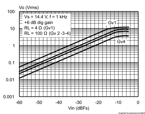
Figure 12. V_o vs. V_{in} (Gv1-2-3-4 settings + 6 dB dig. gain)
