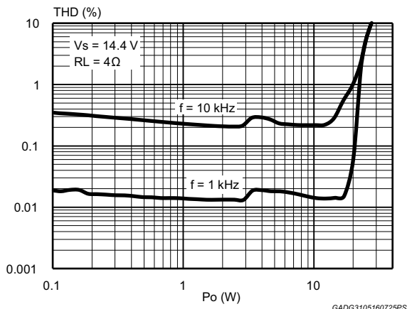
Figure 8. Distortion vs. output power (4 \Omega , SBI mode)
