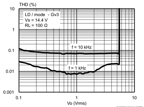
Figure 14. Distortion vs. output voltage (LD-Gv3)
