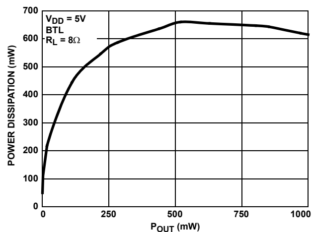
FIGURE 8. POWER DISSIPATION vs OUTPUT POWER
