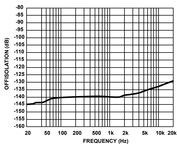
FIGURE 6. OFFISOLATION vs FREQUENCY
