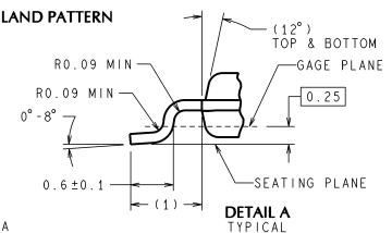
DETAIL A TYPICAL
