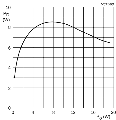
Fig 14. Total (worst case, both channels driven) power dissipation as function of channel output power per channel.
