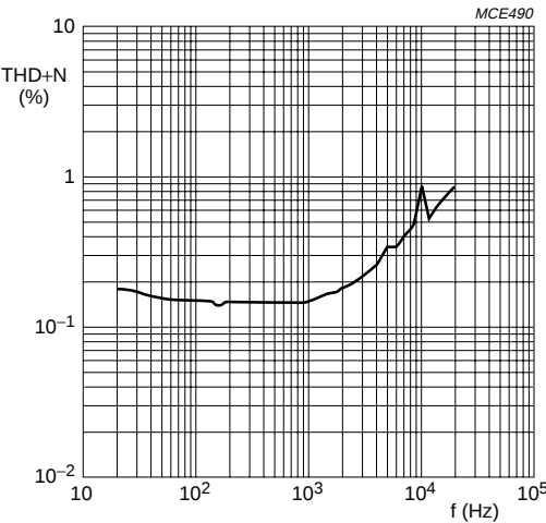
Fig 10. Total harmonic distortion as function of frequency.
