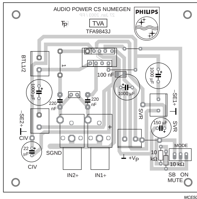
Fig 21. Printed-circuit board layout (single-sided); components view.
