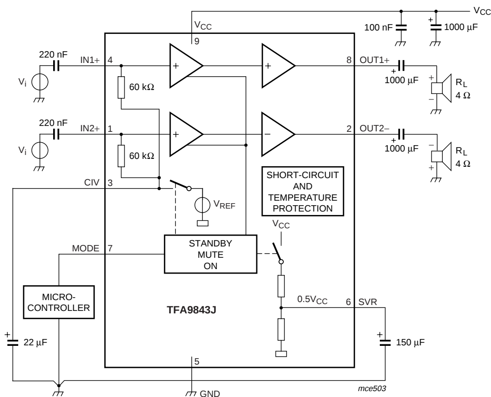
Fig 19. SE application diagram.
