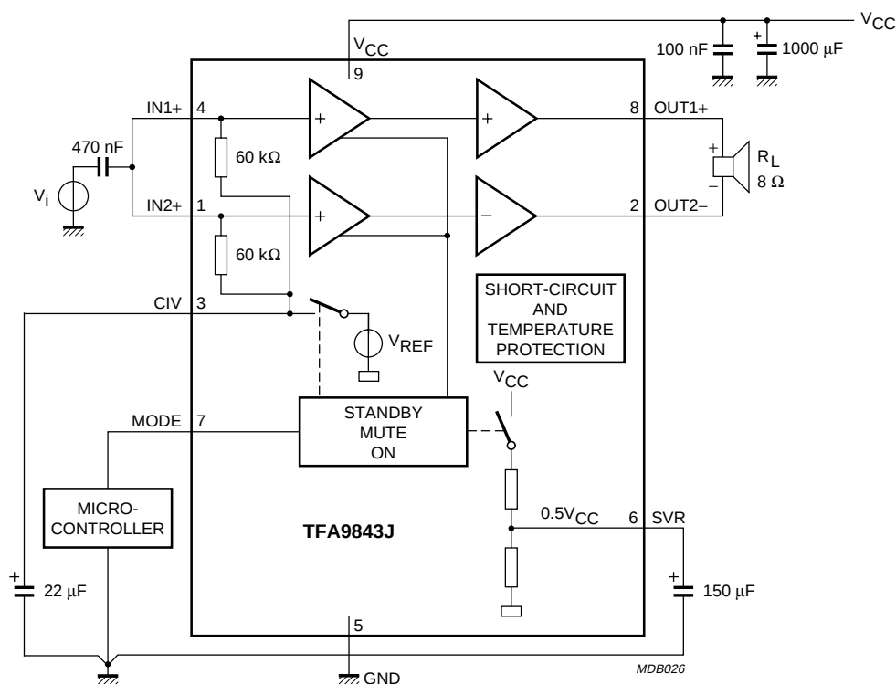
Fig 20. BTL application diagram.
