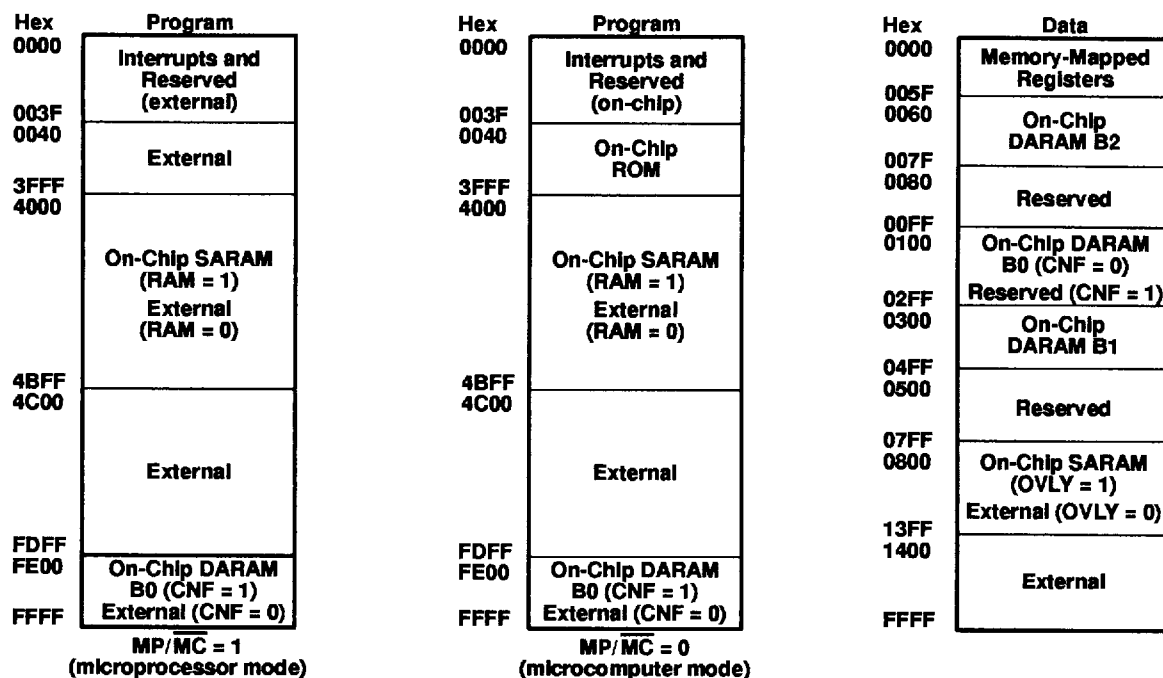
Figure 4. TMS320C53, TMS320C53S, TMS320LC53, and TMS320LC53S Memory Map
