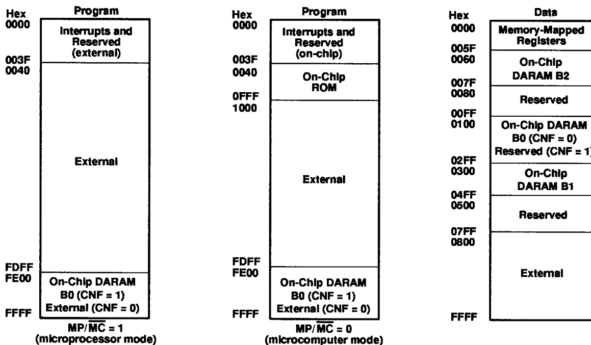
Figure 3. TMS320C52 and TMS320LC52 Memory Map
