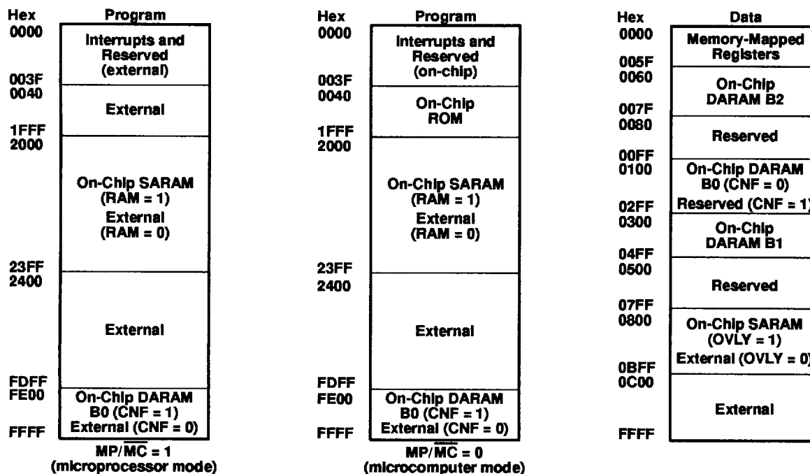
Figure 2. TMS320C51 and TMS320LC51 Memory Map
