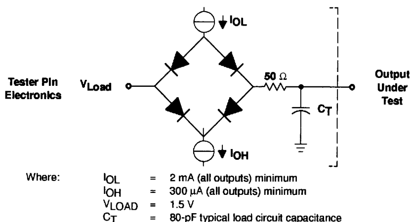
Figure 9. Test Load Circuit
