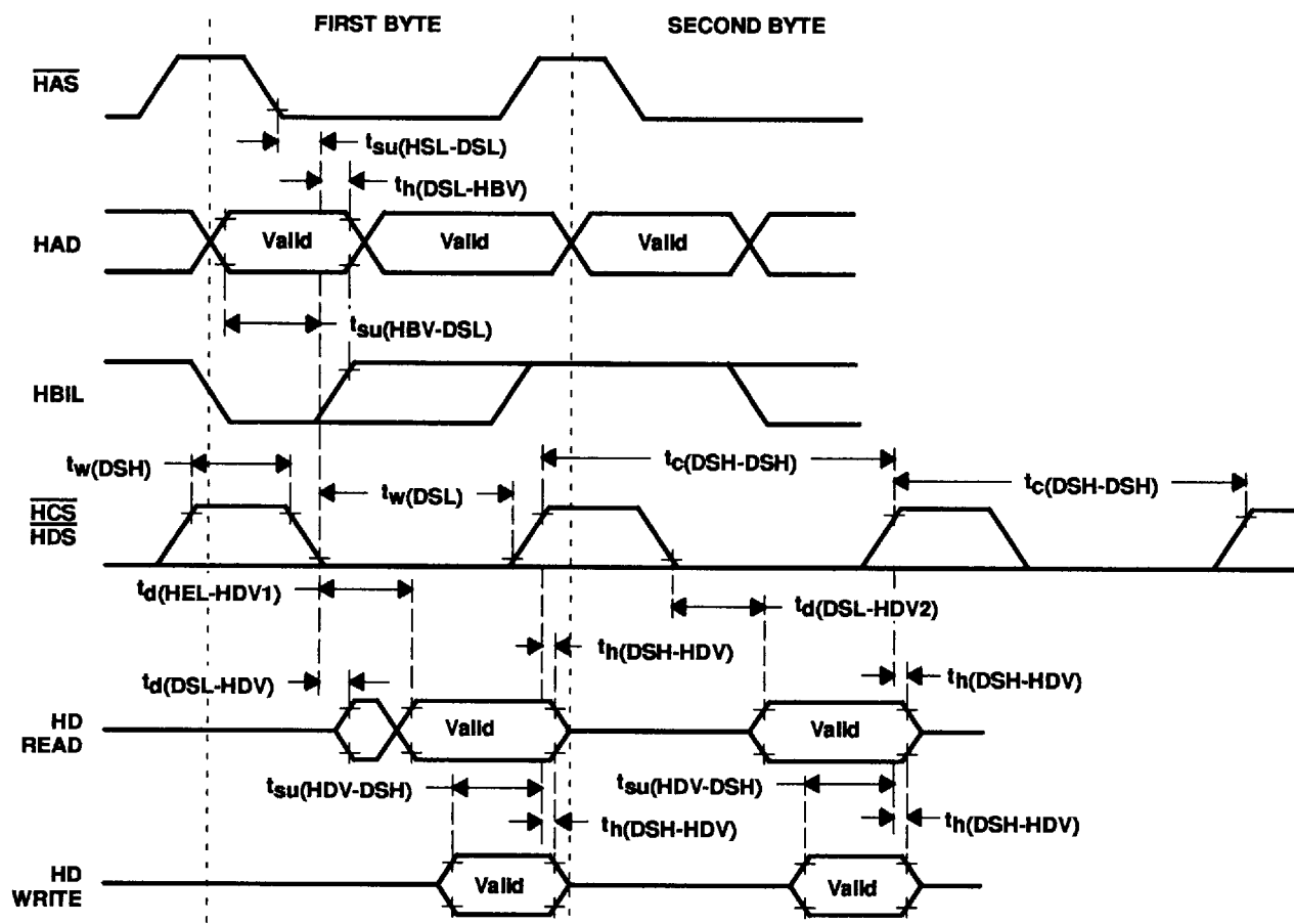
Figure 31. Read/Write Access Timings Using \overline{HAS} Without HRDY
