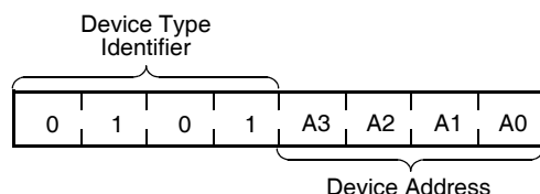
Figure 1. Address/Identification Byte Format
