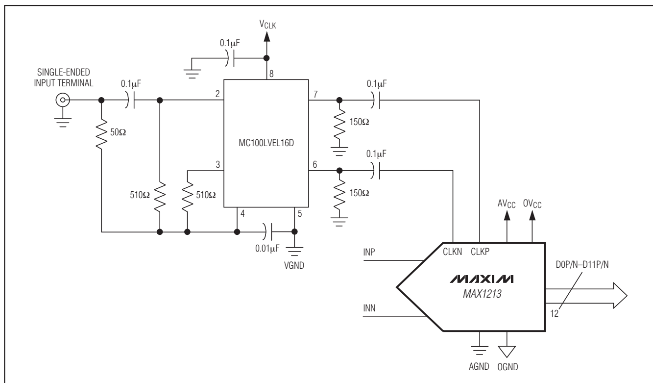
Figure 7. Differential, AC-Coupled, LVPECL-Compatible Clock Input Configuration
