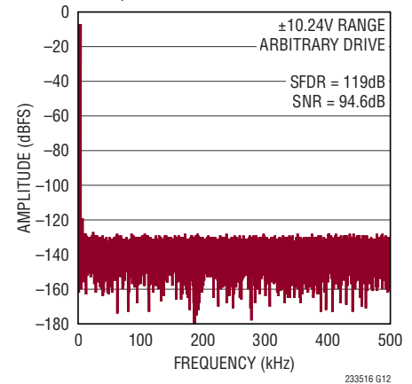
32k Point Arbitrary Two-Tone FFT f_{SMPL} = 1\text{Mps} , IN^+ = -7\text{dBFS} 2kHz Sine, IN^- = -7\text{dBFS} 3.1kHz Sine
