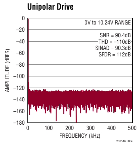
Figure 6e. IN^+ = -1\text{dBFS} 2kHz Unipolar Sine, IN^- = 0\text{V} , 32k Point FFT, f_{\text{SAMPL}} = 1\text{Msps} . Circuit Shown in Figure 6a with LT1358 Amplifiers, R_{\text{FILT}} = 100\Omega , C_{\text{FILT}} = 270\text{pF}
