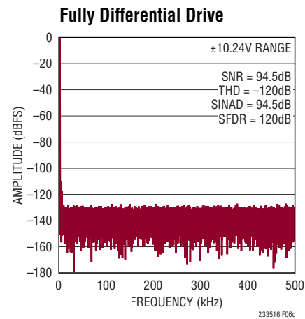
Figure 6c. IN^+/IN^- = -1\text{dBFS} 2kHz Fully Differential Sine, V_{\text{CM}} = 0\text{V} , 32k Point FFT, f_{\text{SAMPL}} = 1\text{Msps} . Circuit Shown in Figure 6a with LT1358 Amplifiers, R_{\text{FILT}} = 100\Omega , C_{\text{FILT}} = 270\text{pF}
