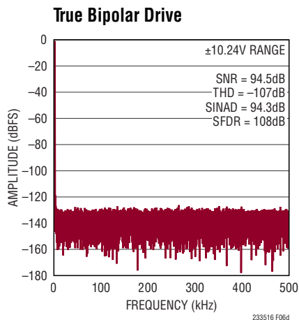
Figure 6d. IN^+ = -1\text{dBFS} 2kHz True Bipolar Sine, IN^- = 0\text{V} , 32k Point FFT, f_{\text{SAMPL}} = 1\text{Msps} . Circuit Shown in Figure 6a with LT1358 Amplifiers, R_{\text{FILT}} = 100\Omega , C_{\text{FILT}} = 270\text{pF}
