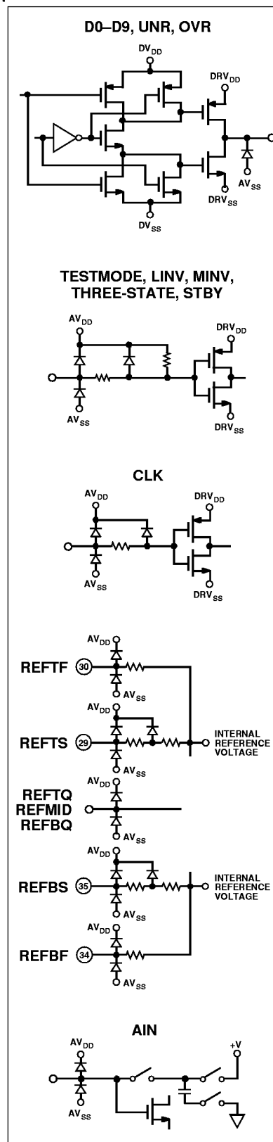
Equivalent Circuits
