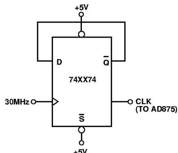
Figure 12. Divide-By-Two Clock Input Circuit
