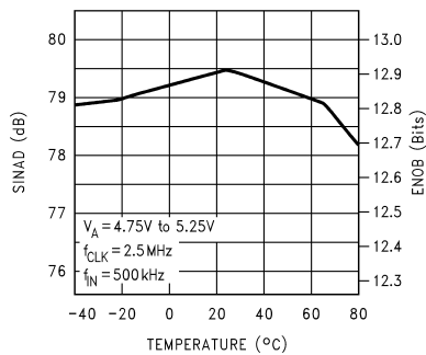
SINAD &amp; ENOB vs Temperature
