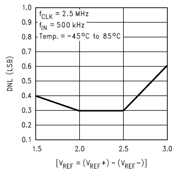
DNL vs V_{REF} and Temperature
