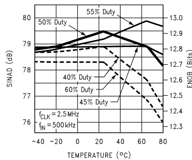
SINAD &amp; ENOB vs Clock Duty Cycle
