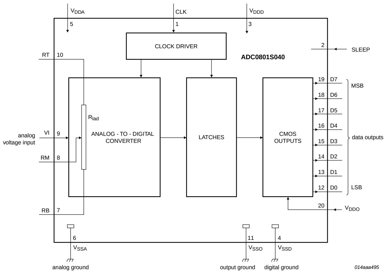
Fig 1. Block diagram
