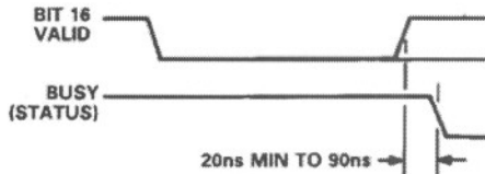
Figure 9. LSB Valid to Status Low
