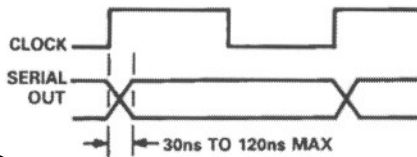
Figure 10. Clock High to Serial Out Valid
