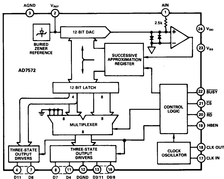
Q Package (DIP)
