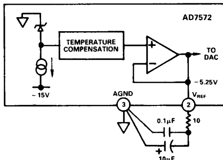
Figure 9. AD7572 Internal -5.25 \text{ V} Reference
