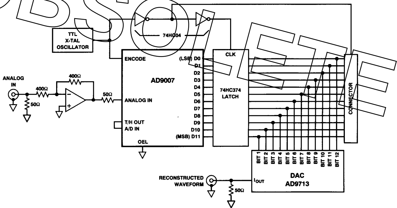
Figure 5. Evaluation Circuit
