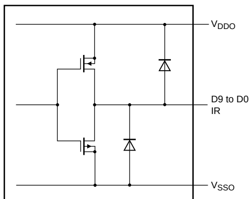
Fig 10. D9 to D0 and IR outputs
