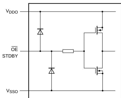
Fig 12. OE and STDBY inputs
