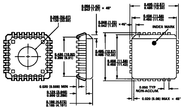
28-Pin PLCC Package
