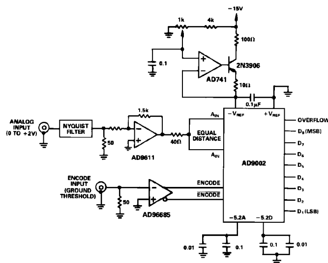
Typical AD9002 Application
