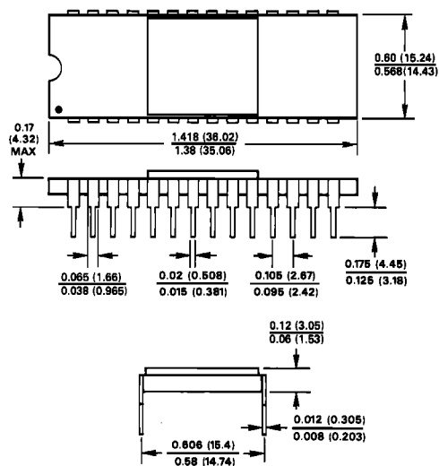
28-Pin Ceramic Side-Brazed DIP
