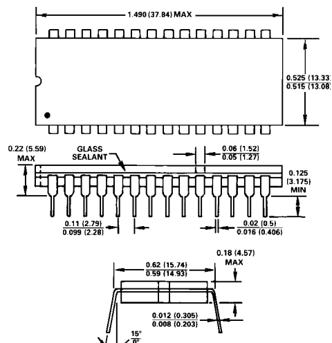
28-Pin Cerdip
