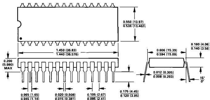
28-Pin Plastic DIP Package
