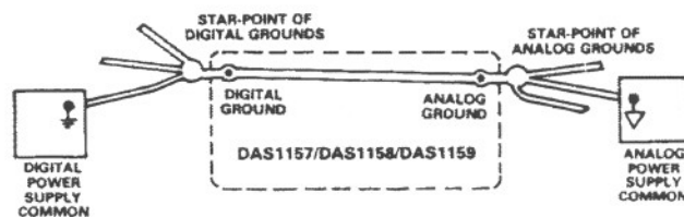
Figure 4. Typical Ground Layout for DAS1157/DAS1158/DAS1159
