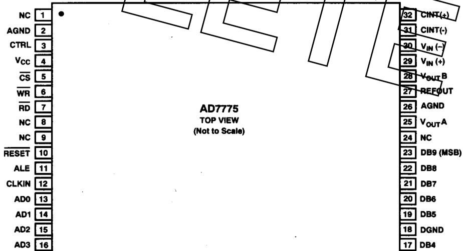
AD7775 TSOP
