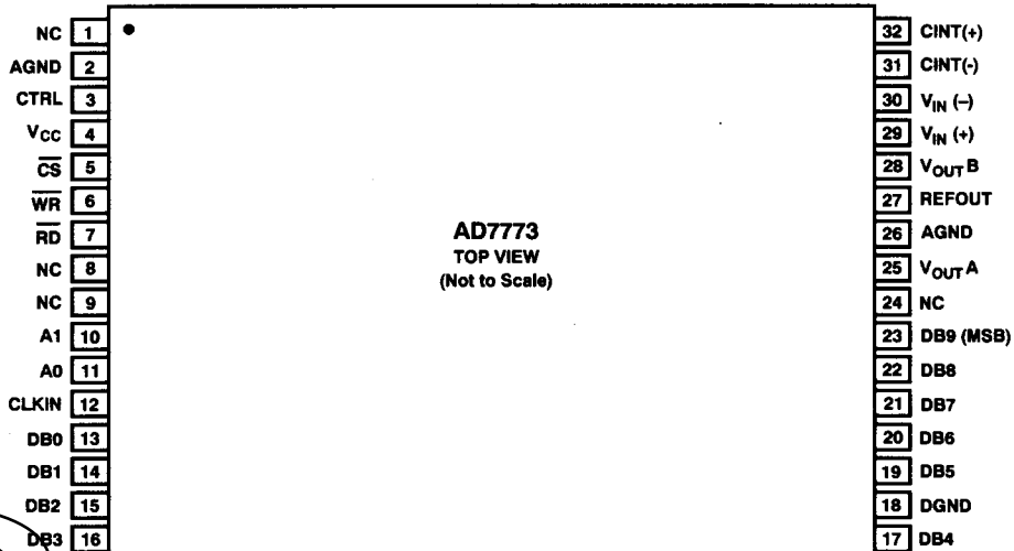
AD7773 TSOP
