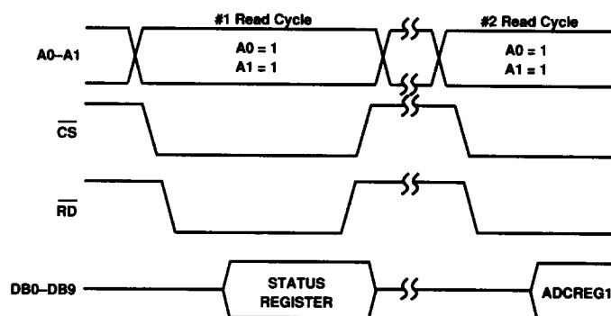
Figure 12a. AD7773 Stack Read Option 1
