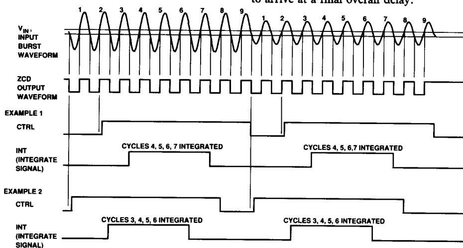
Figure 21. Two Examples of Movement of the Integration Window as a Result of Relative Timing Between CTRL and the Input Burst Signal
