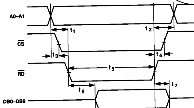
Figure 1. Read Cycle Timing for AD7773 Interface
