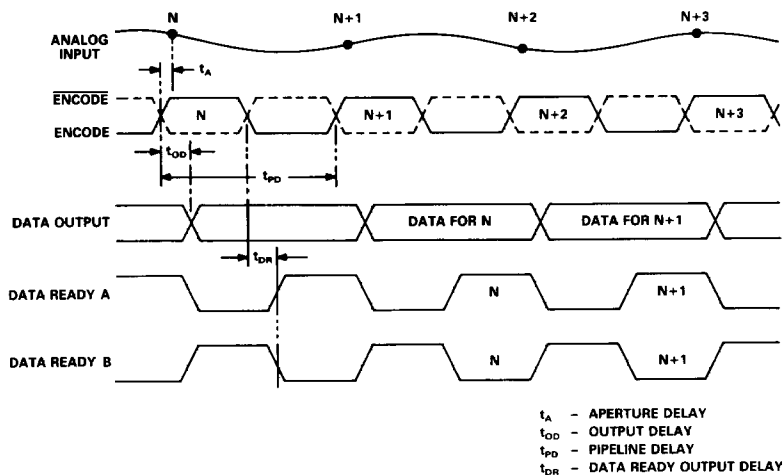
AD9028 Timing Diagram
