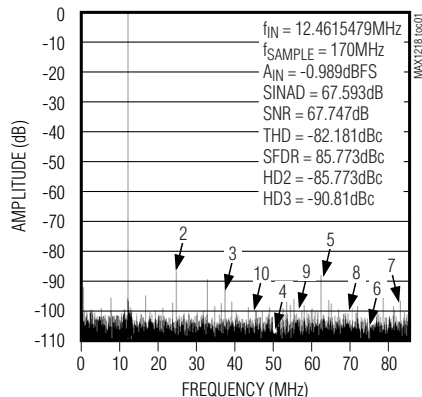
FFT PLOT (16,384 SAMPLES)
