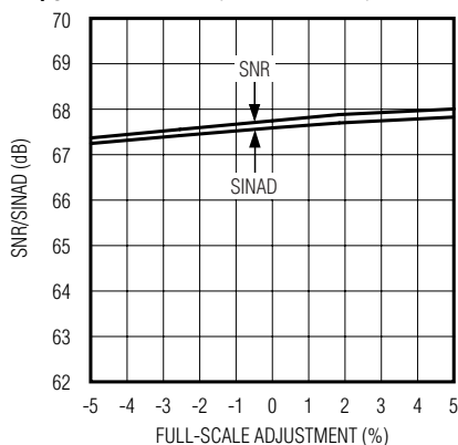
SNR/SINAD vs. % FS ADJUSTMENT ( f_{SAMPLE} = 170MHz , f_{IN} = 12.5MHz , A_{IN} = -1dB )
