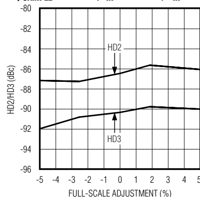
HD2/HD3 vs. % FS ADJUSTMENT ( f_{SAMPLE} = 170MHz , f_{IN} = 12.5MHz , A_{IN} = -1dBFS )
