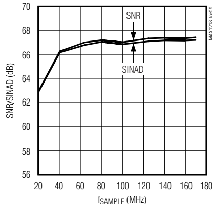
SNR/SINAD vs. SAMPLE FREQUENCY ( f_{IN} = 64.9847412MHz , A_{IN} = -1dBFS )
