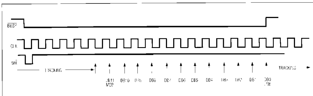
Figure 6. MAX182 Timing Diagram
