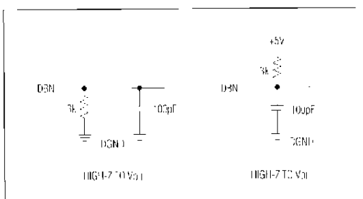
Figure 3 Load Circuits for Access Time Test ( t_1 )
