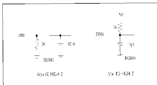
Figure 4 Load Circuits for Output Three-State Delay Test ( t_2 )
