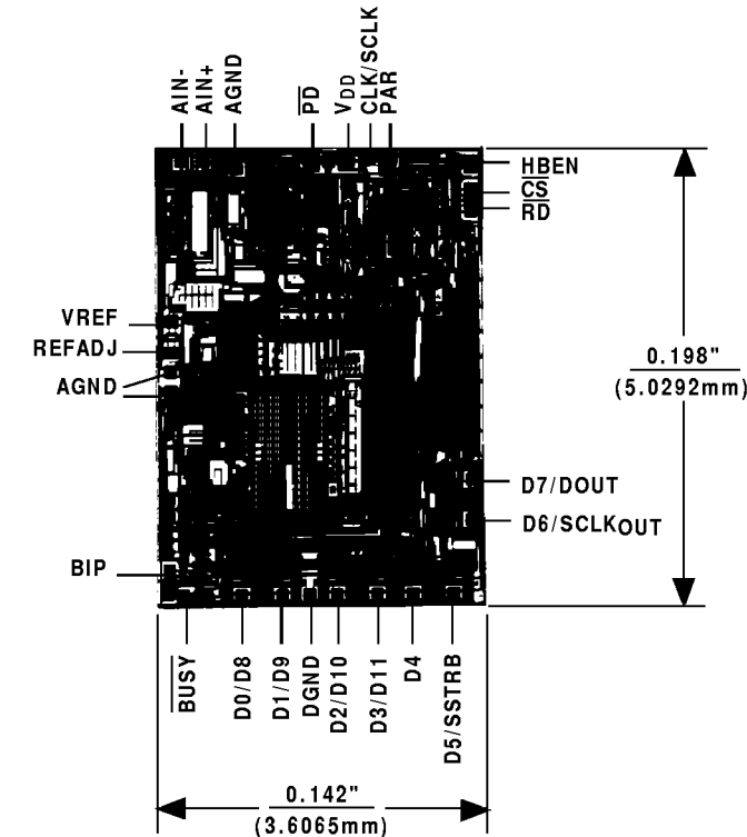
Chip Topography
