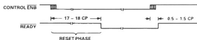
Figure 14b. Timing Diagram for Disabling and Enabling Controller Using CONTROL \overline{\text{ENB}} (RST = 1)
