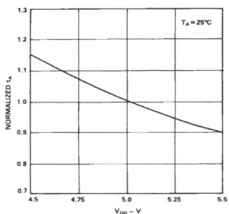
Figure 10. Normalized Data Access Time vs. V_{DD}
