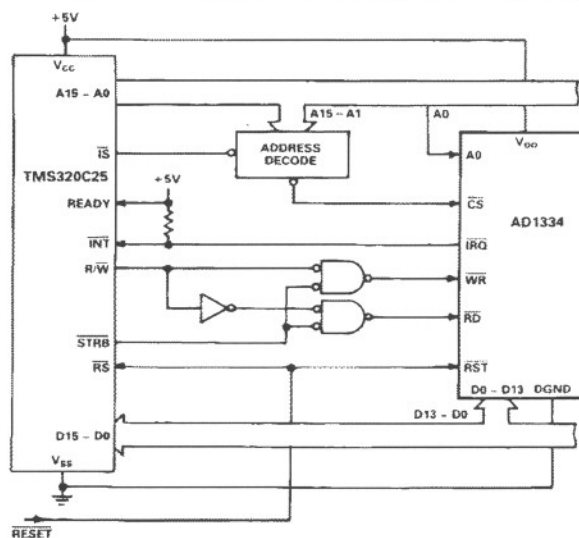
Figure 18. TMS320C25 to AD1334 Interface
