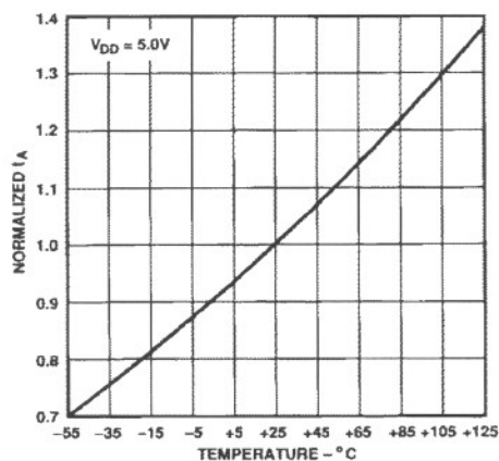
Figure 11. Normalized Data Access Time vs. Temperature
