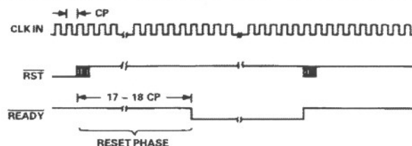
Figure 14a. Timing Diagram for Resetting Controller (CONTROL \overline{\text{ENB}} = 0)
