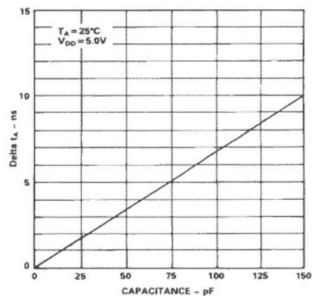
Figure 12. Change in Data Access Time vs. Loading
