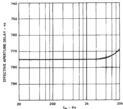
Figure 6. Effective Aperture Delay vs. Frequency
