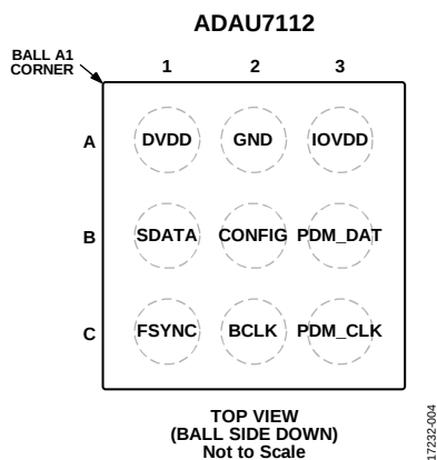
Figure 4. Pin Configuration
