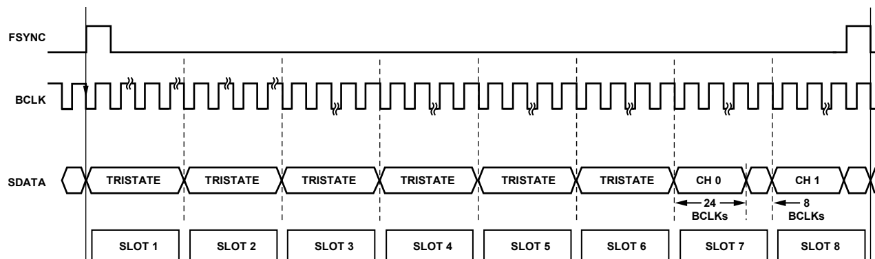
Figure 17. TDM-8, BCLK = 256 \times f_s , CONFIG Pin Tied to GND Through a 47 k \Omega Resistor
