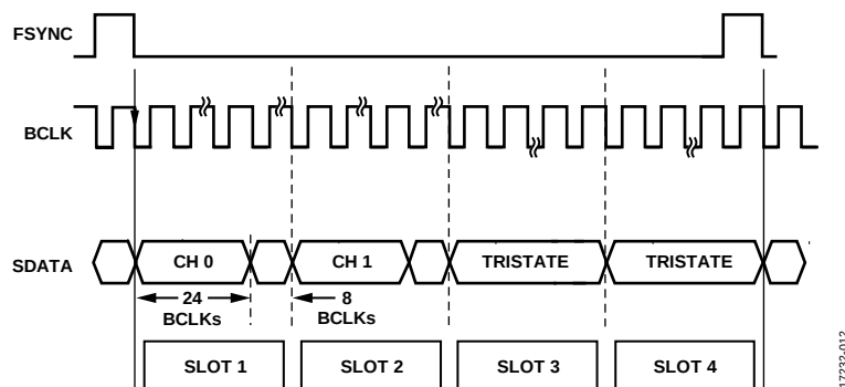
Figure 12. TDM-4, BCLK = 128\times f_s , CONFIG Pin Tied to GND
