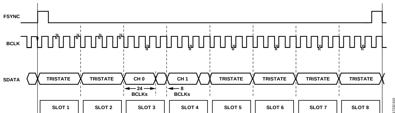
Figure 15. TDM-8, BCLK = 256 \times f_s , CONFIG Pin Open
