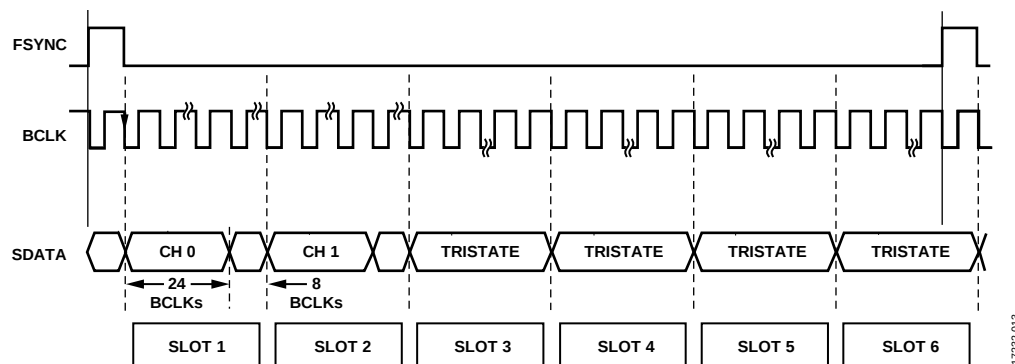
Figure 13. TDM-6, BCLK = 192 \times f_s , CONFIG Pin Tied to GND
