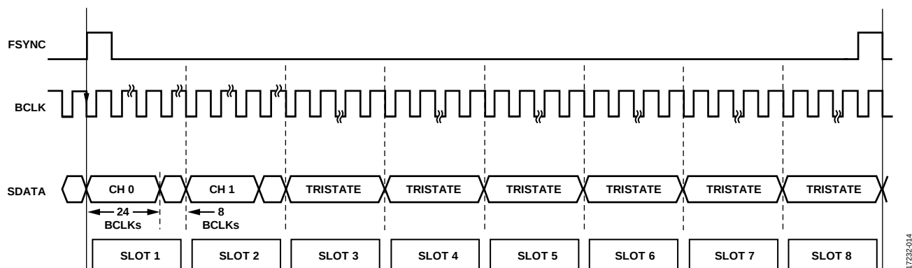
Figure 14. TDM-8, BCLK = 256 \times f_s , CONFIG Pin Tied to GND
