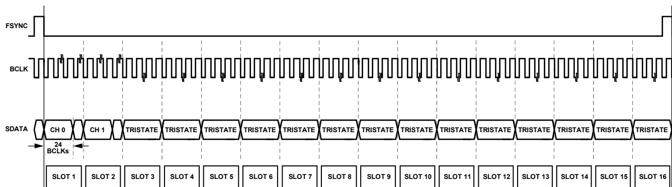
Figure 19. TDM-16, BCLK = 512 \times f_s , CONFIG Pin Tied to GND
