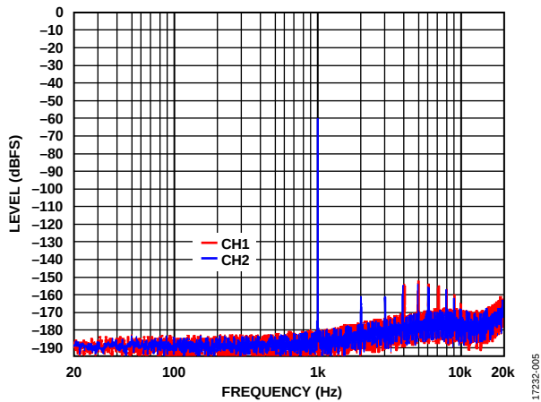
Figure 5. Fast Fourier Transform (FFT), f_s = 48 kHz, -60 dBFS Input, 64\times Decimation, Fifth Order
