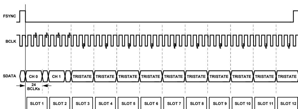
Figure 18. TDM-12, BCLK = 384 \times f_s , CONFIG Pin Tied to GND
