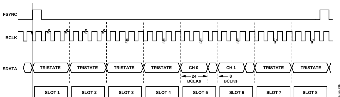
Figure 16. TDM-8, BCLK = 256 \times f_s , CONFIG Pin Tied to IOVDD Through a 47 k \Omega Resistor
