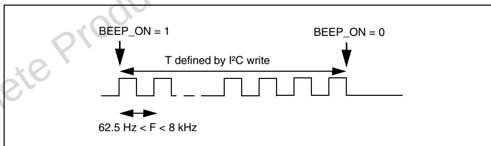
Figure 14: Continuous Mode
