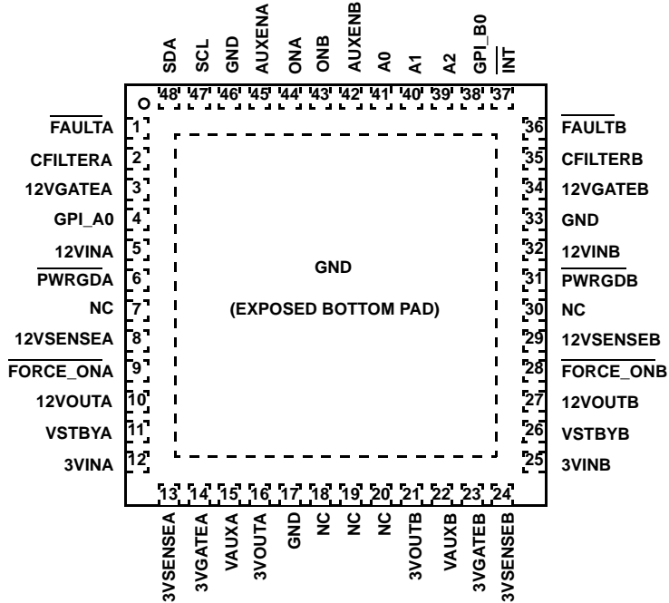
ISL6112 (48 LD 7X7 QFN) TOP VIEW
