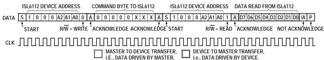
FIGURE 18. READ_BYTE PROTOCOL
