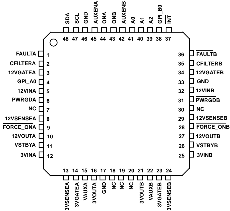
ISL6112 (48 LD 7X7 TQFP) TOP VIEW
