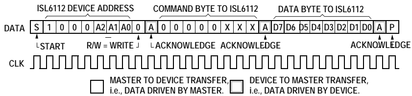
FIGURE 17. WRITE_BYTE PROTOCOL
