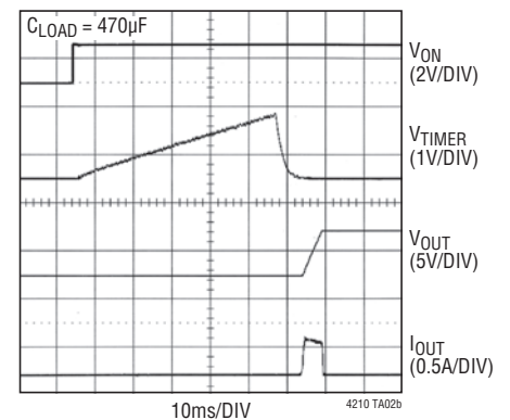
Power-Up Sequence
